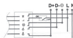
C. Dimming function
