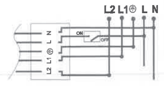
D. Multiple loop function
